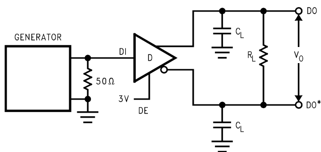
Figure 5. Driver I_{OD}
